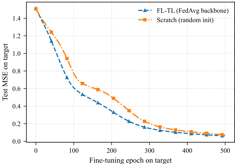
Scenario 4.2: TL on GFLI7 (FL vs Scratch)
