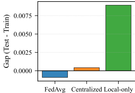
(c) Overfitting gap
