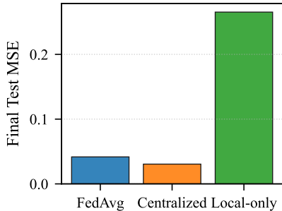
(a) Final performance
