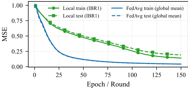
IBR1: local-only vs FedAvg
