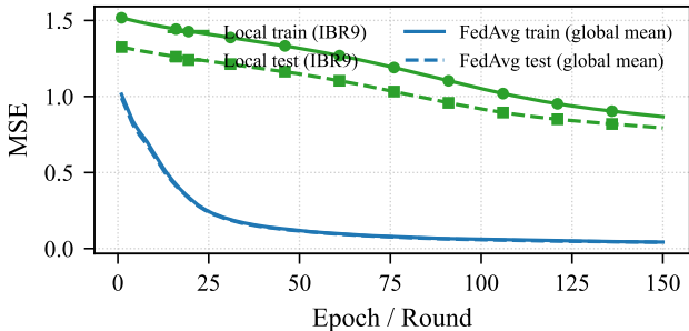
IBR9: local-only vs FedAvg
