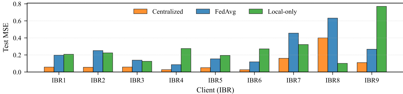
Per-IBR Test Performance
