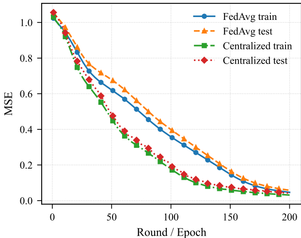
Training & test performance
