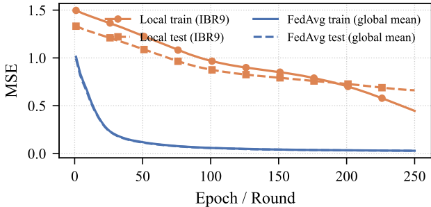
IBR9: train & test curves
