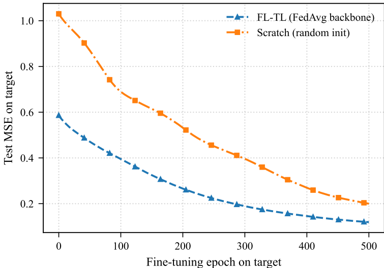
Scenario 4.2: TL on GFLI1 (FL vs Scratch)
