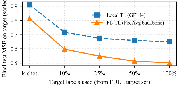
Data efficiency on IBR1 (FL-TL vs Local TL)
