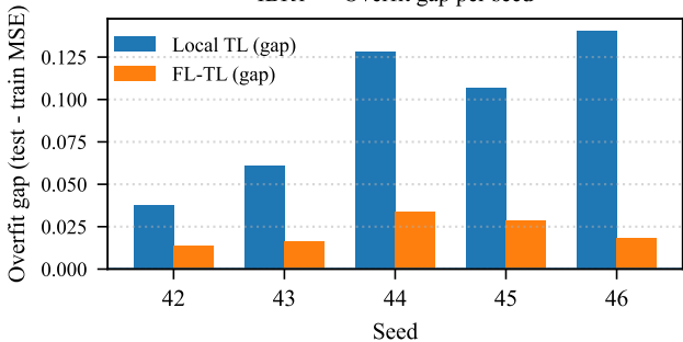
IBR1 — Overfit gap per seed
