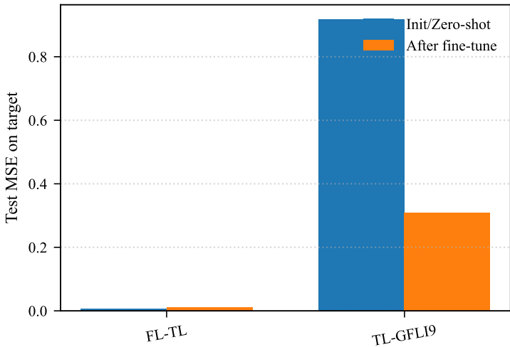
Init vs fine-tuned performance (anti-overfit)
