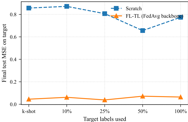
Data efficiency on GFLI9 (Central TL removed)
