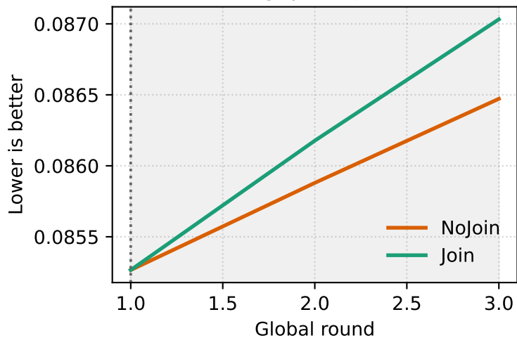
Fairness gap: 1 - Jain index
