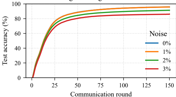
Scenario F: FedAvg Learning Curves Across Noise Levels
