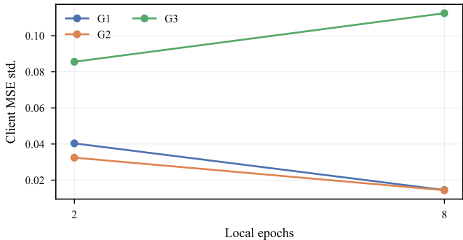
Fairness vs local epochs
