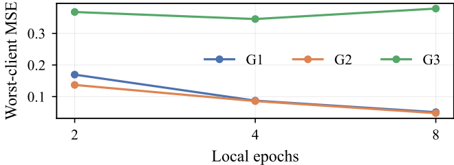
Worst client vs local epochs
