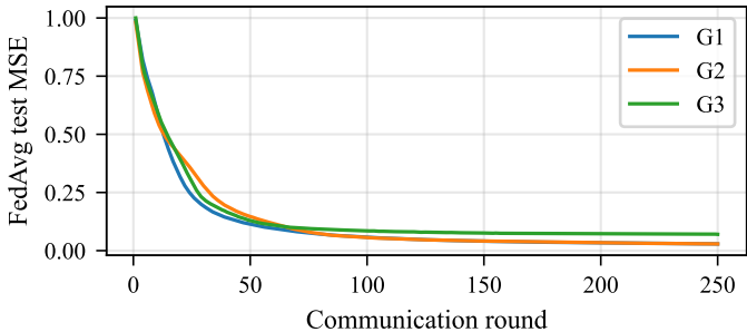
FedAvg learning curves
