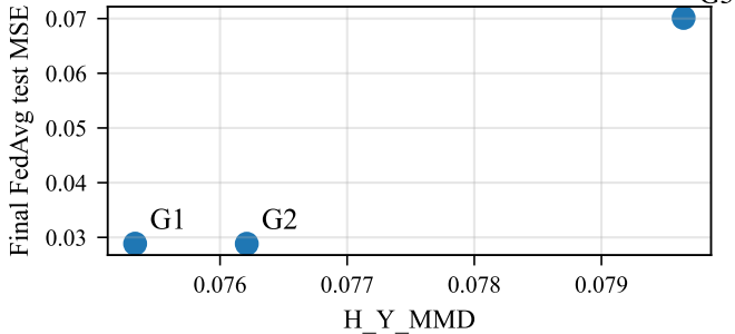
Final MSE vs heterogeneity
