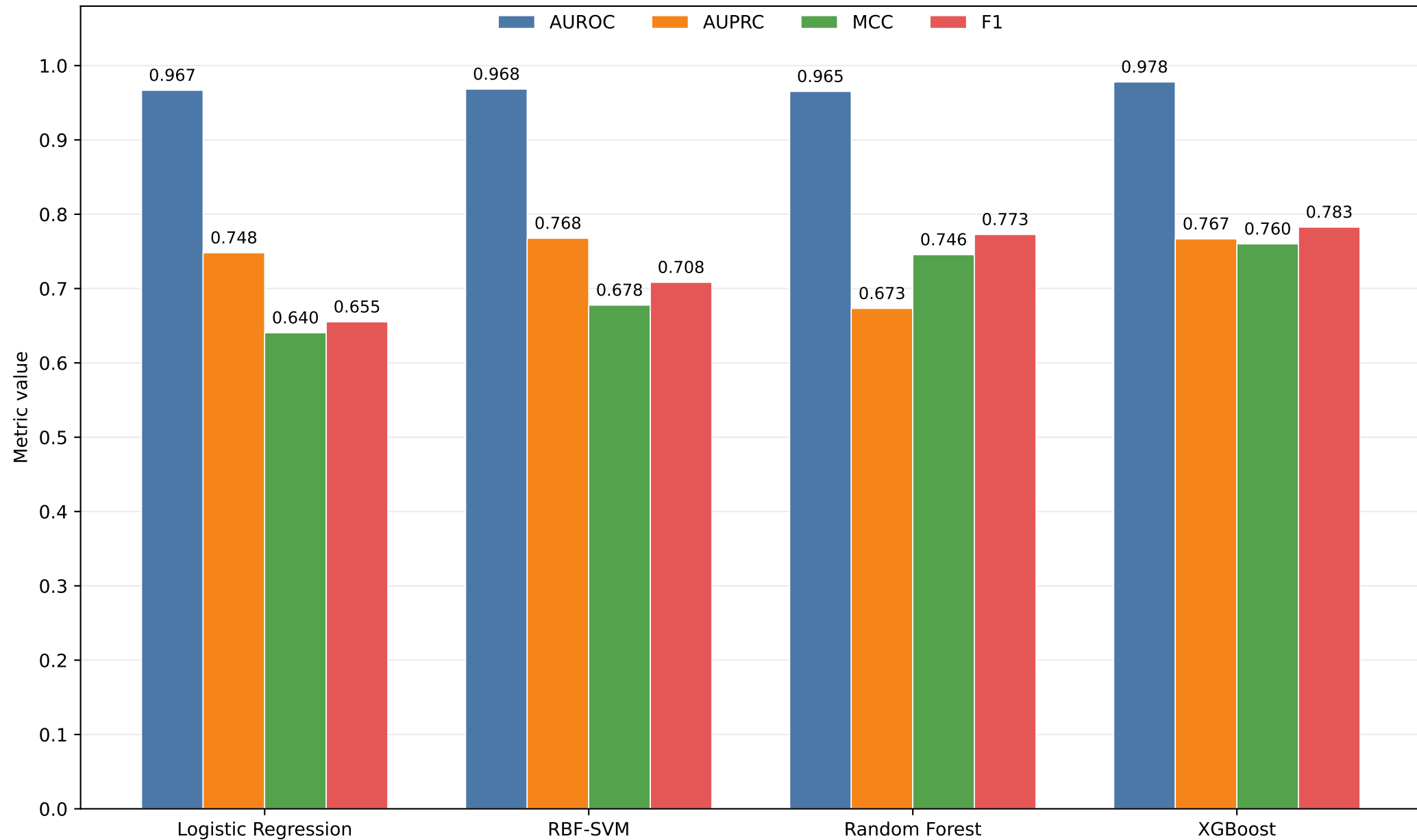
Traditional-model metric comparison
