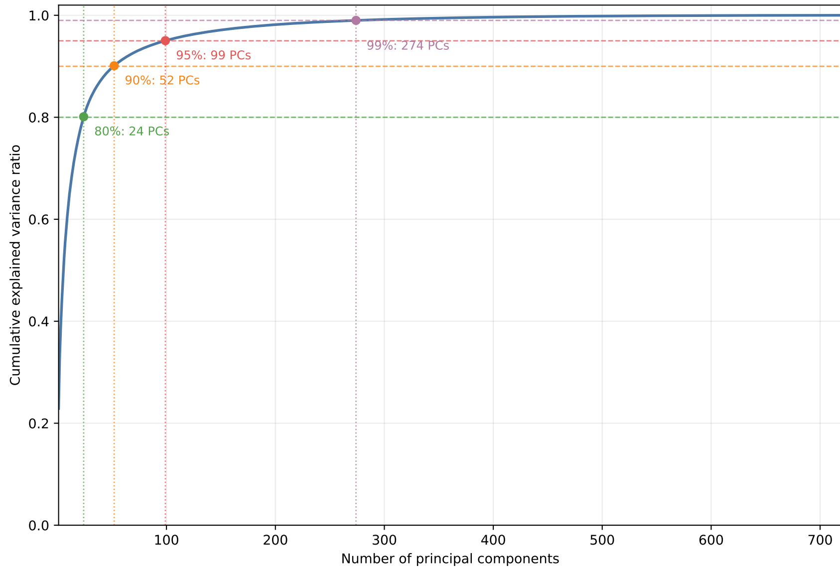
Development-only standardized ESM-2 PCA
