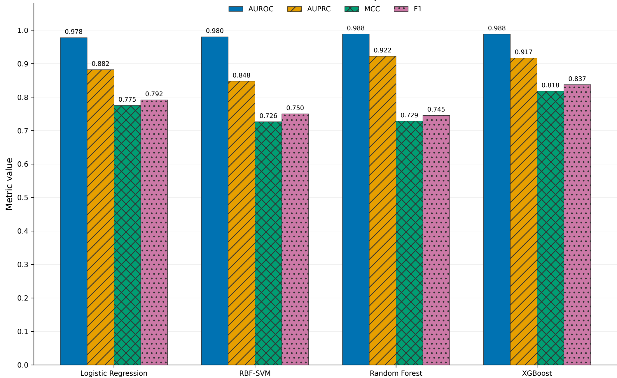
ESM-2 model metric comparison
