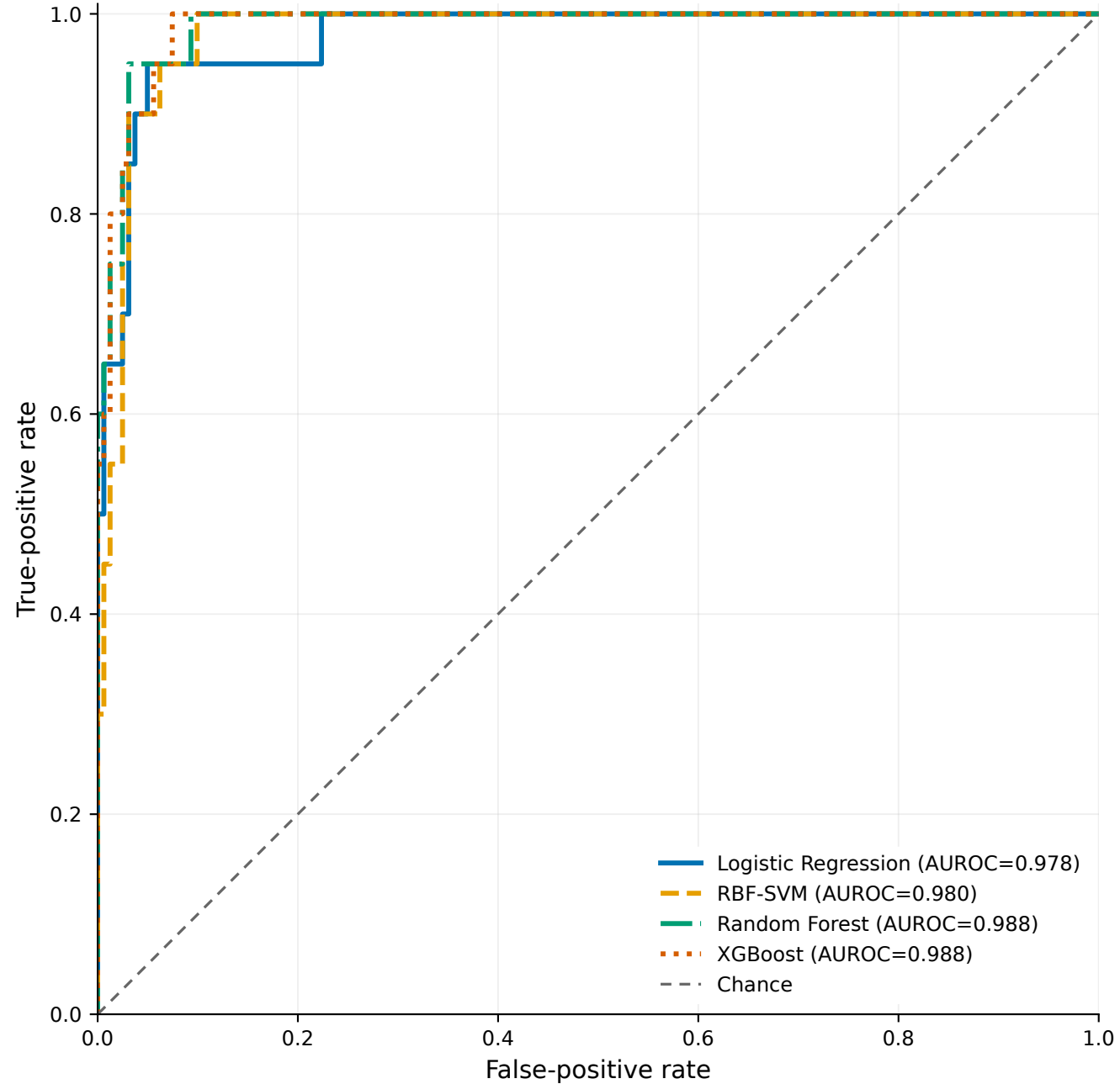
ESM-2 model ROC curves
