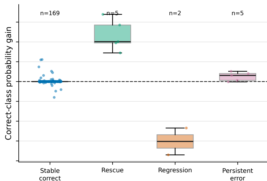
D XGBoost
