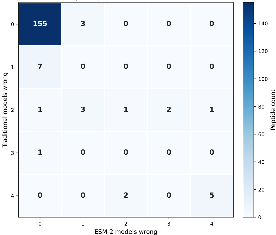
Overlap of representation-level test errors
