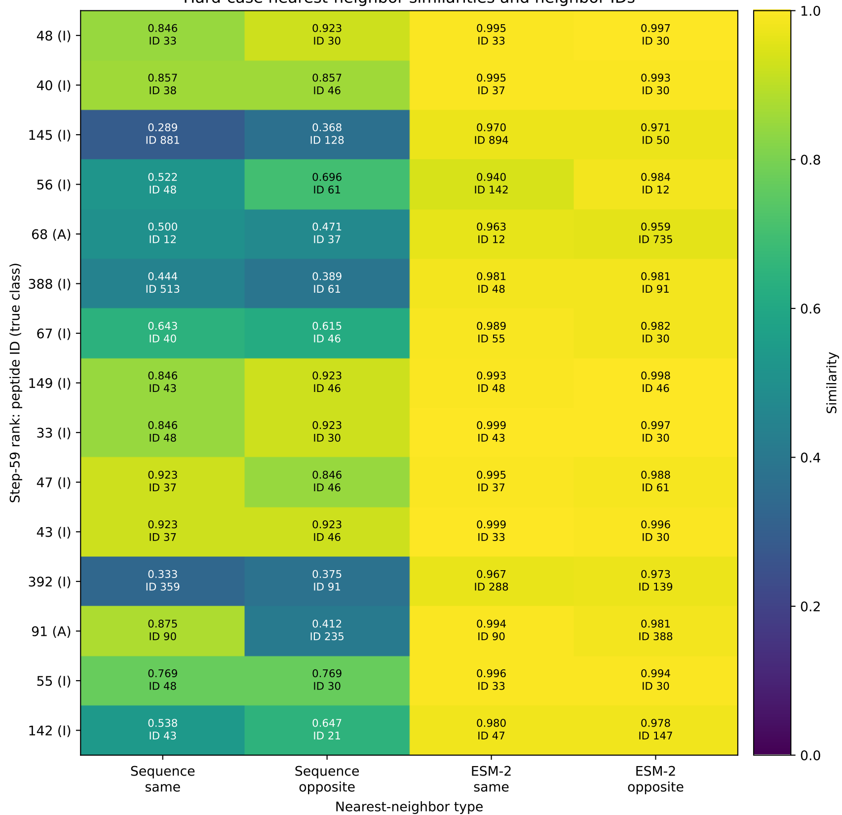
Hard-case nearest-neighbor similarities and neighbor IDs
