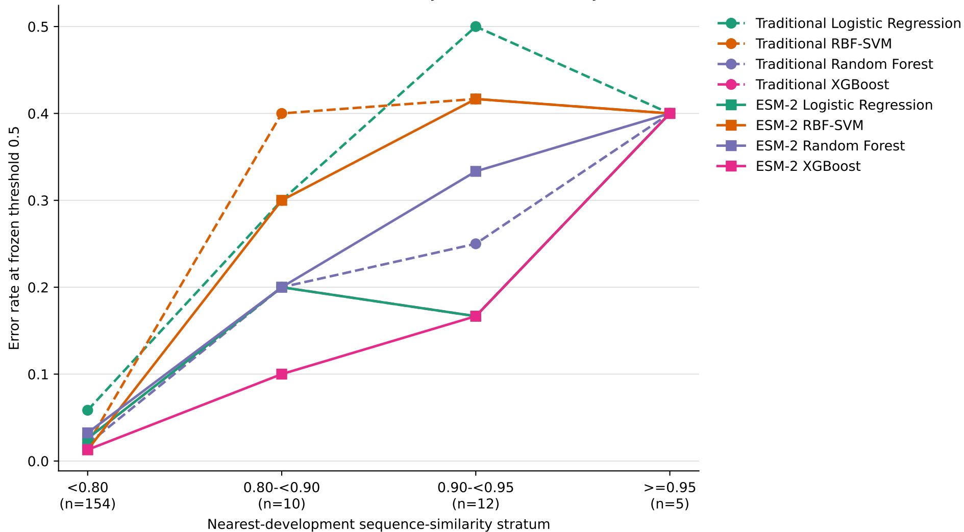
Frozen-model error rates across mutually exclusive similarity strata
