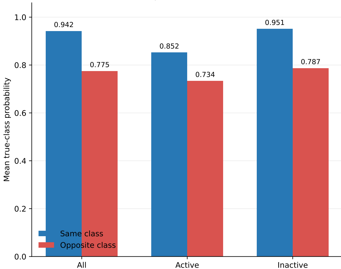
Frozen prediction confidence
