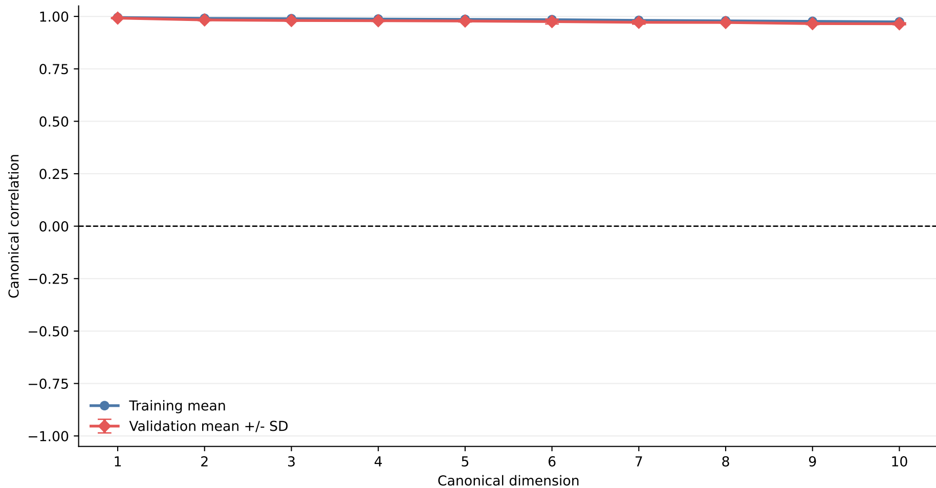
Cross-Validated Traditional-ESM-2 Canonical Correlations
