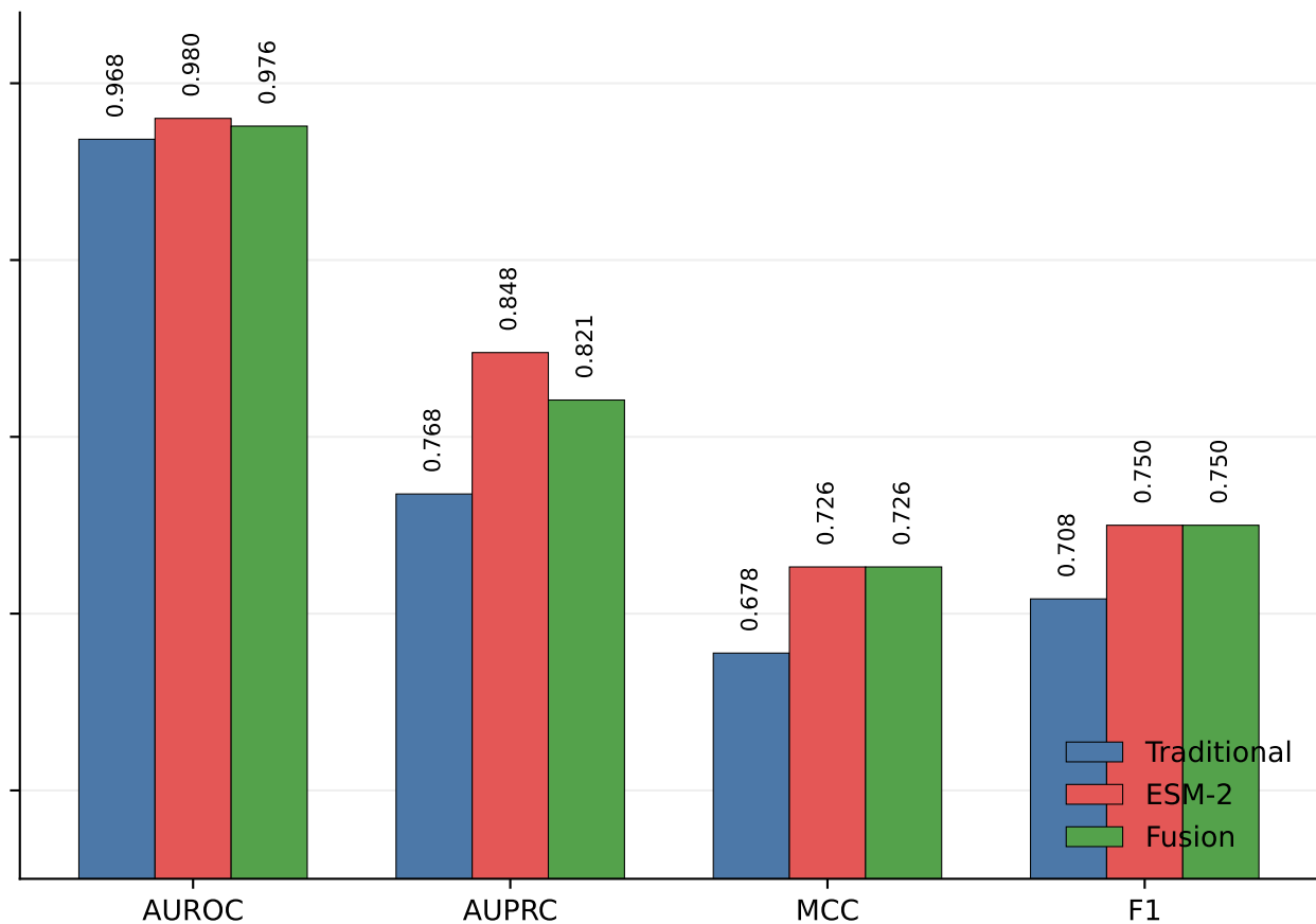
B RBF-SVM
