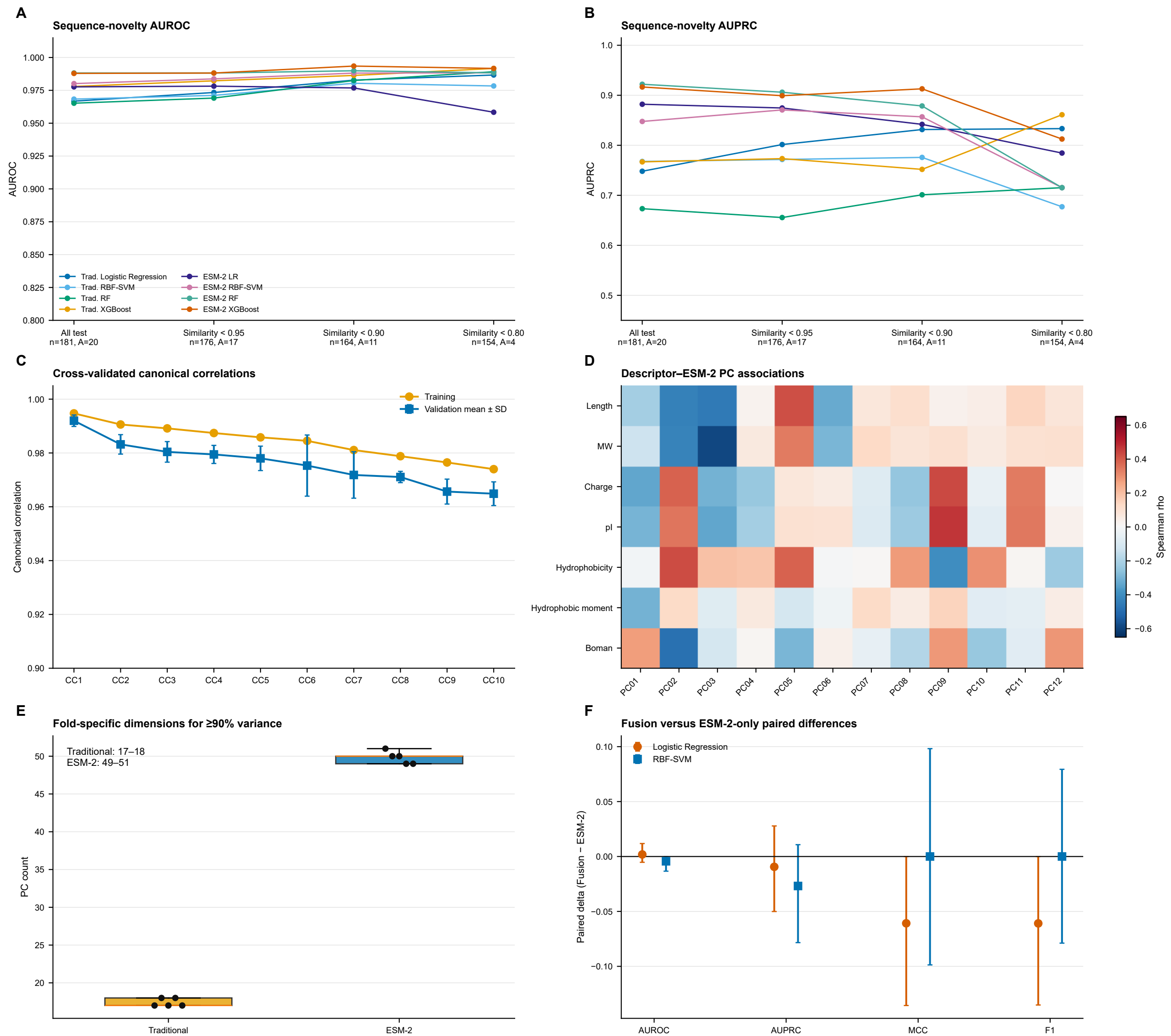
Figure 3. Generalization, sequence novelty, and representation complementarity
