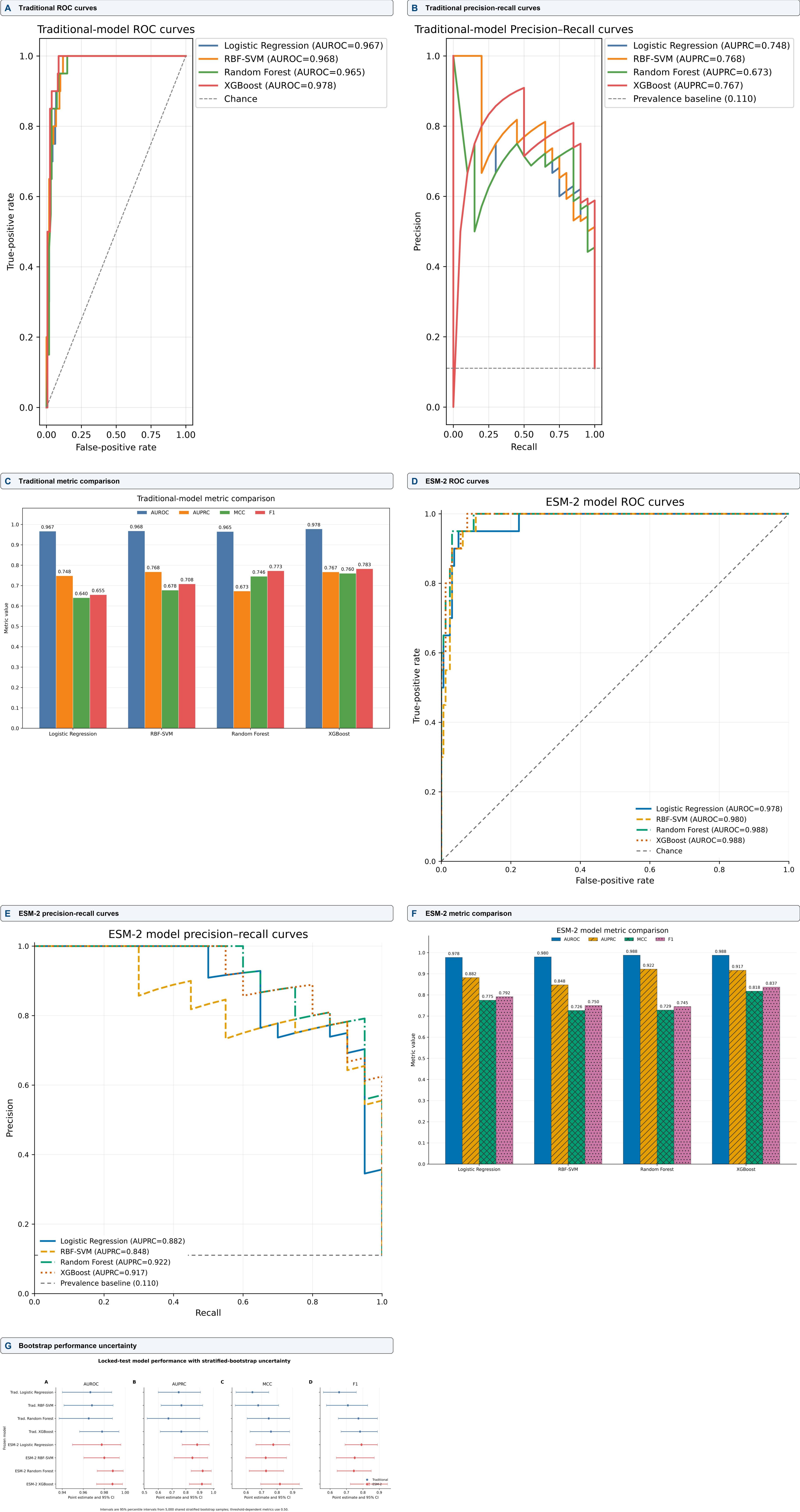
Figure 2. Traditional and ESM-2 predictive performance
