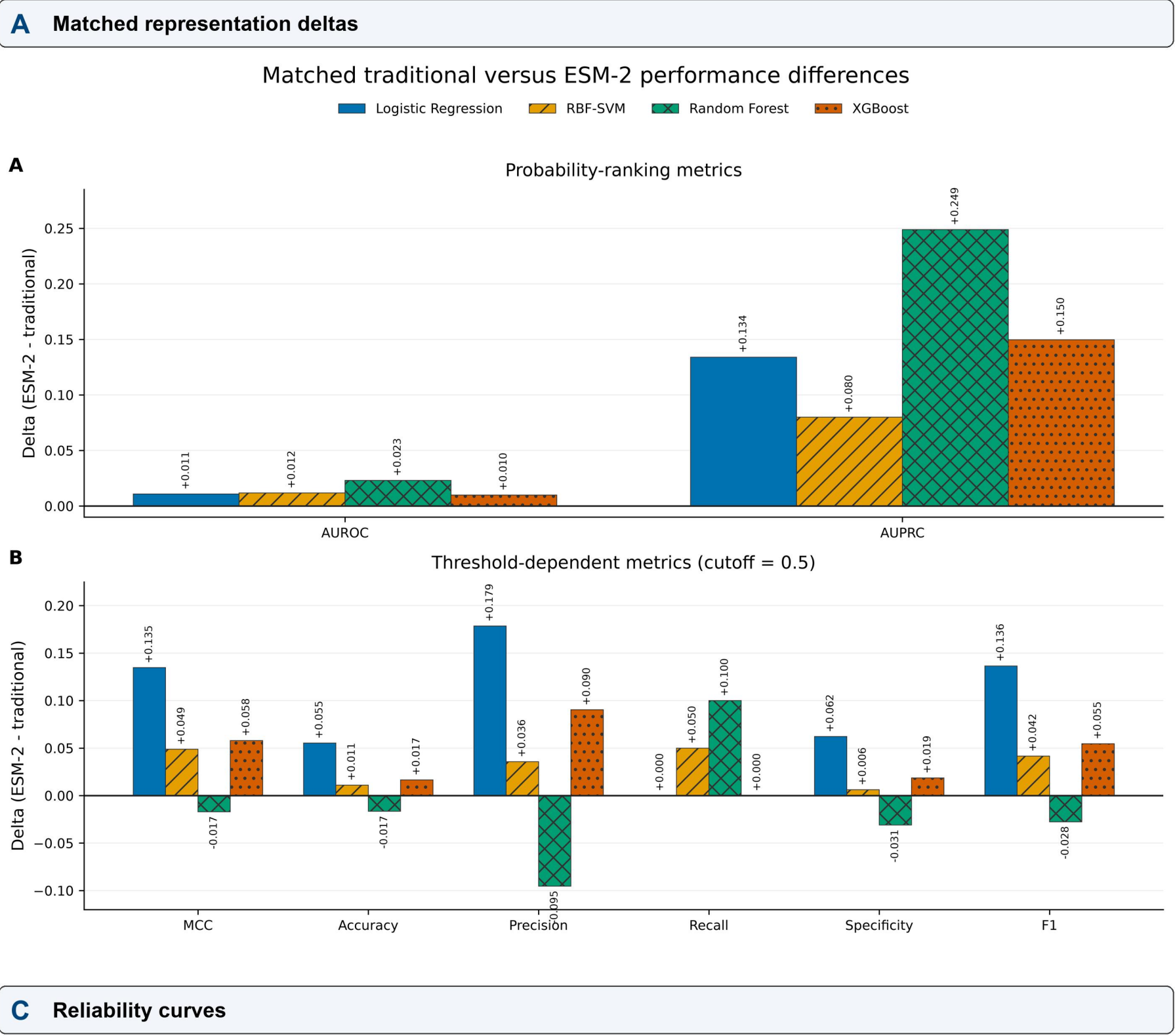
Figure 3. Matched improvements, calibration, and decision utility
