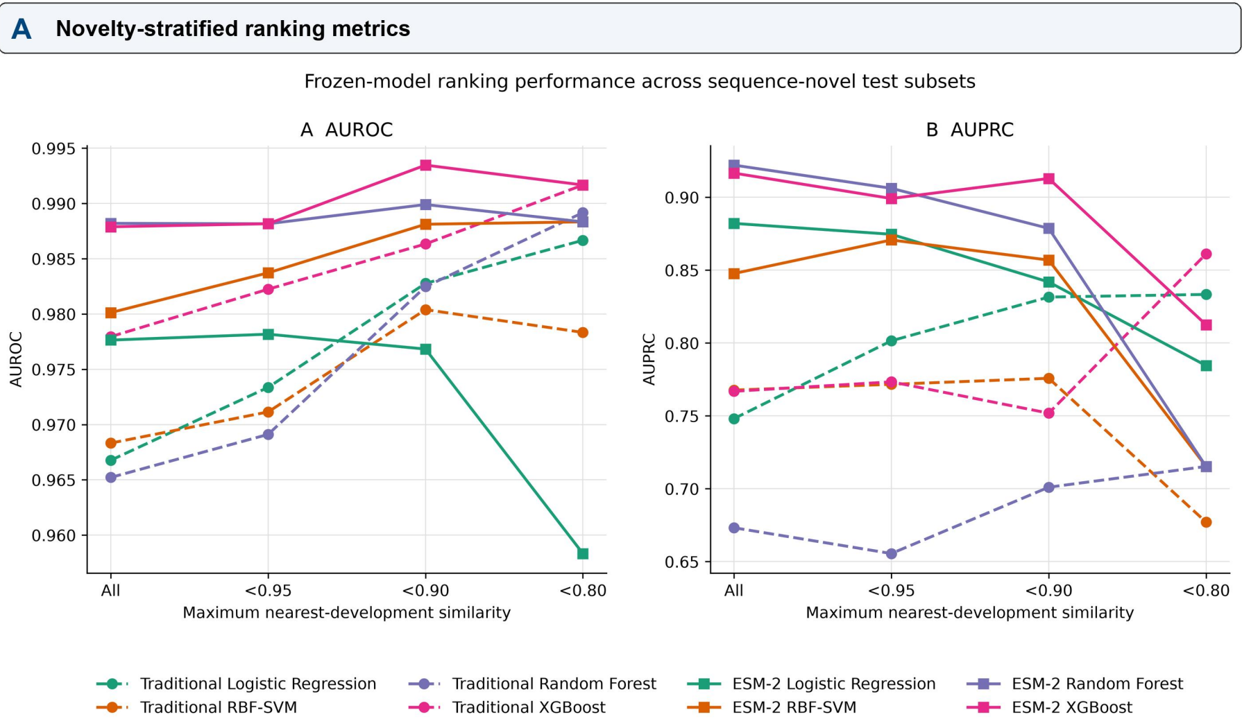
Figure 4. Sequence novelty and homology-aware generalization
