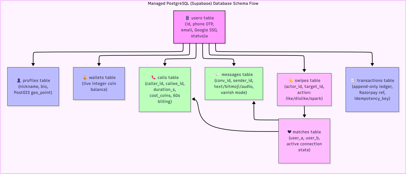
Figure 2: YoUnMe Managed PostgreSQL (Supabase Pro) Database Schema Flow Diagram
