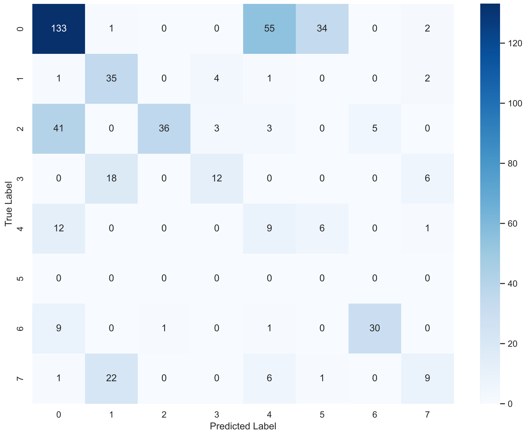
GPT-5 Confusion Matrix - OdinW DroneControl
