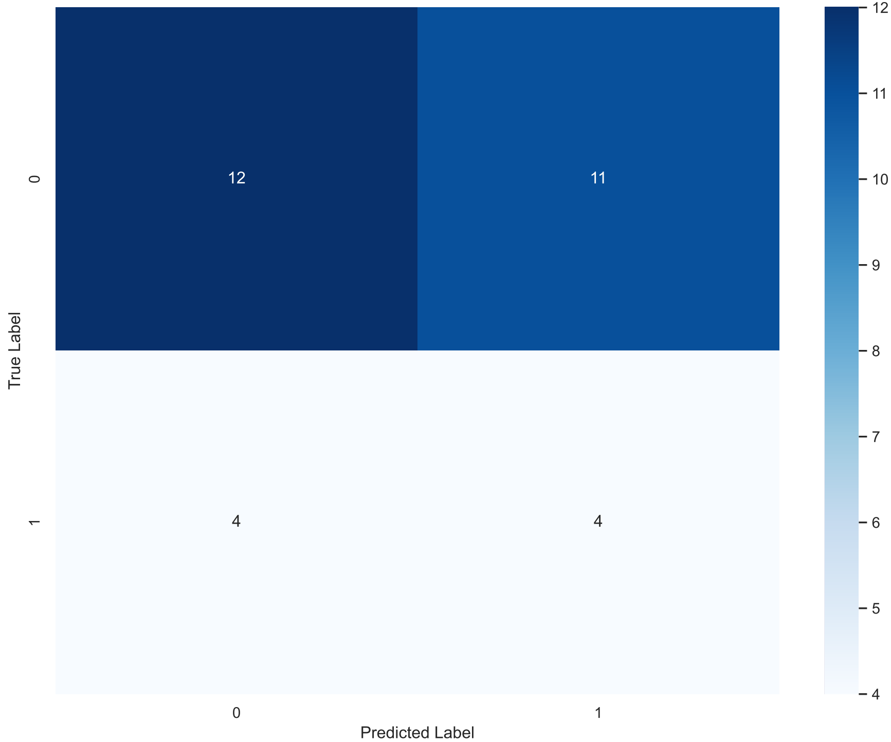
GPT-5 Confusion Matrix - OdinW ThermalCheetah
