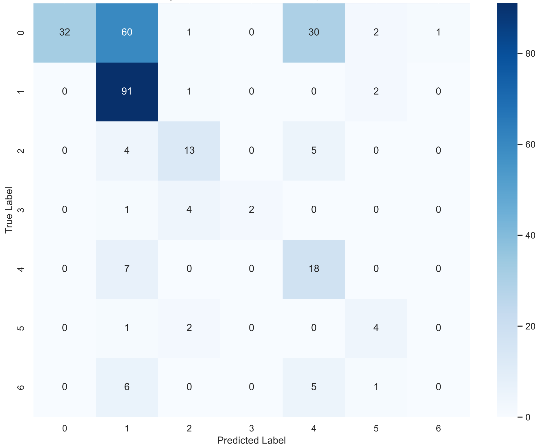
Magma Confusion Matrix - OdinW Aquarium
