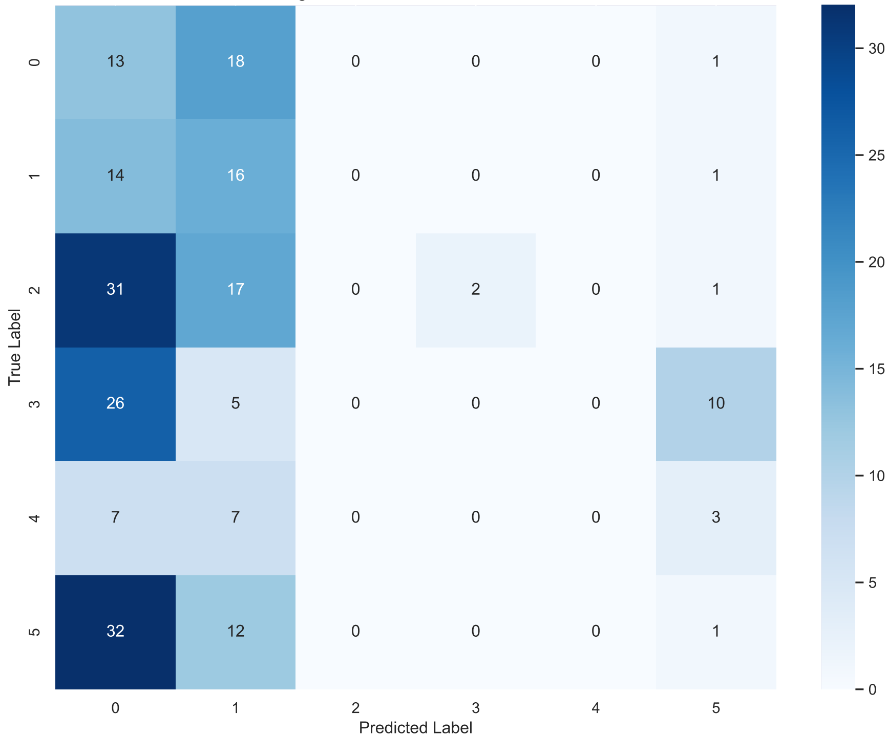
Magma Confusion Matrix - OdinW dice
