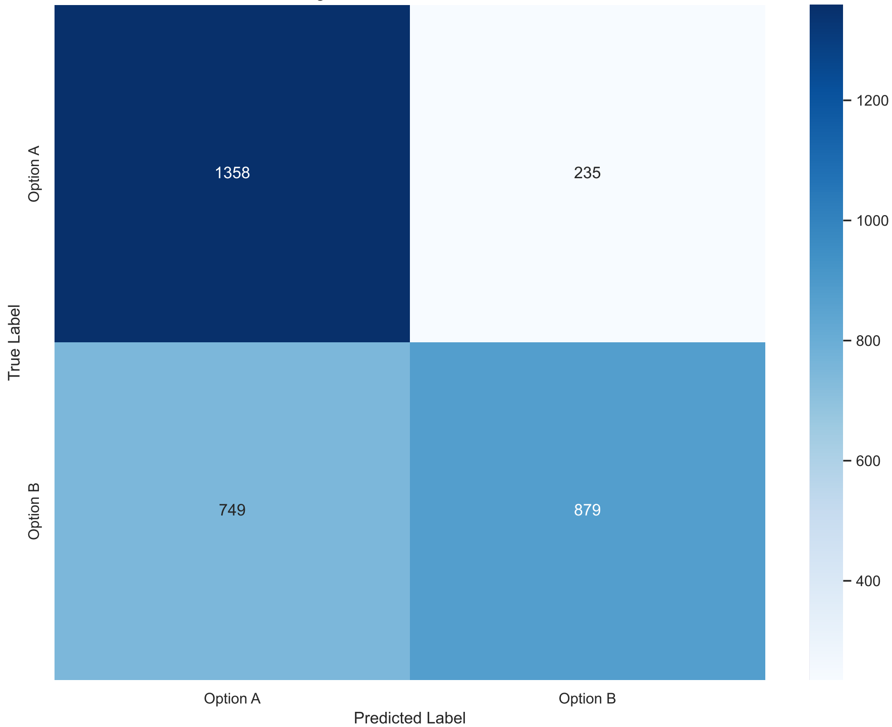
Magma Confusion Matrix - PIQA
