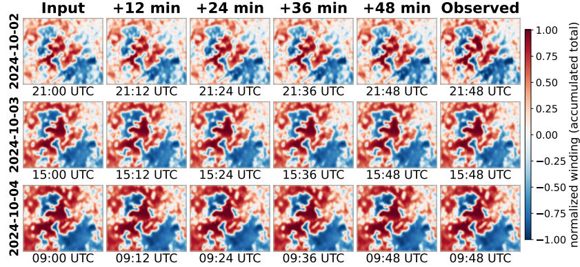
Figure 3.3: Winding-flux forecasts on the held-out active region HARP 11930. Each row is an independent window: the latest input frame, the four autoregressive forecasts at +12, +24, +36, +48 minutes, and the observed frame at +48 minutes, all stamped with their true UTC time. The model is trained only on the other 26 regions.
