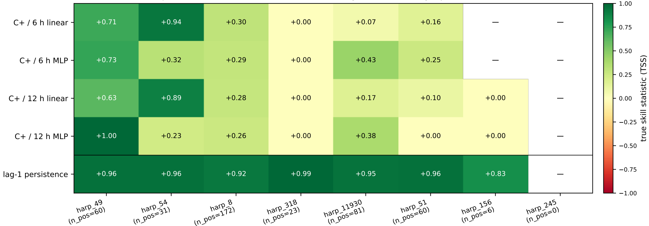
C+ flare classifier: per-cube TSS across four head--window configurations, with lag-1 persistence baseline (bottom row)
