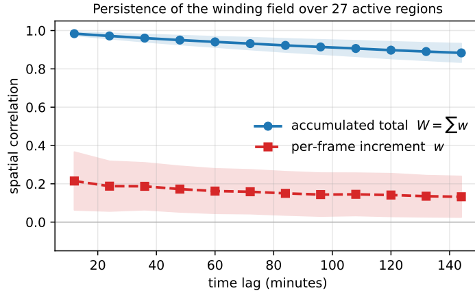
Figure 2.1: The accumulated total winding is smooth and strongly persistent. Spatial correlation between winding frames separated by a given time lag, averaged over the active-region corpus (shaded band: one standard deviation across regions). The accumulated total (blue) remains strongly correlated over hours, decaying only gradually—the property that makes it a well-posed forecasting target. The per-frame increment (red) is shown for contrast. Because the total is so persistent, its forecast skill must be read against a persistence baseline, as it is throughout Chapter 3.
