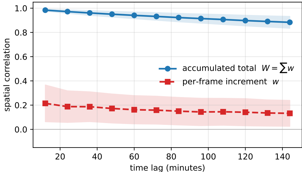
Persistence of the winding field over 27 active regions
