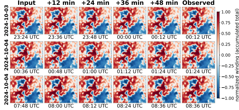
Winding-flux forecast — held-out AR HARP 11930 ( t_{in} = 10 \rightarrow t_{out} = 4 , 12-min cadence)
