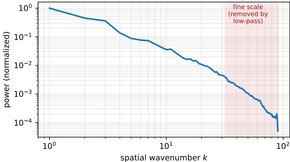
Winding power persists to the smallest spatial scales
