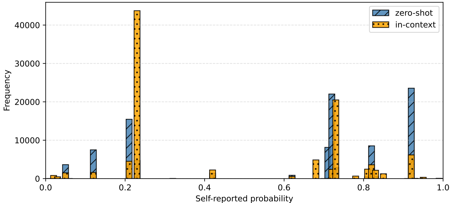
Distribution of Llama-3.3 self-reported probabilities
