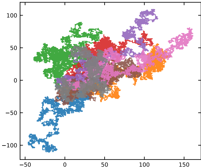
2D Random Walk (10000 steps)
