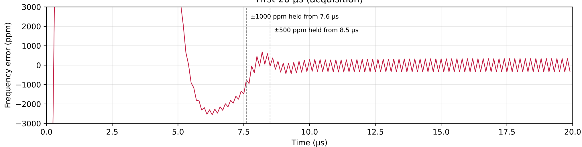
First 20 \mu\text{s} (acquisition)
