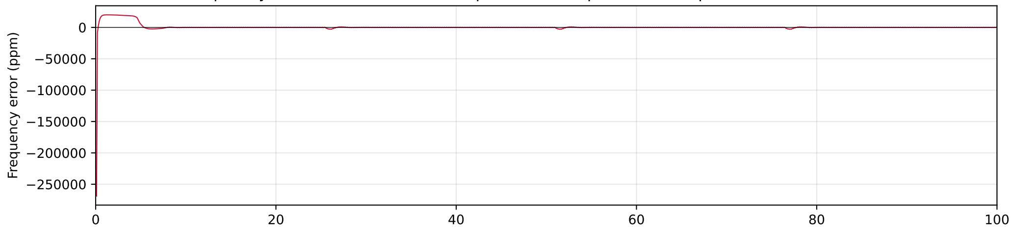
PLL pre-layout: lock over the full 100 \mu\text{s} (one value per reference period, N = 244 , 2.44 GHz)
