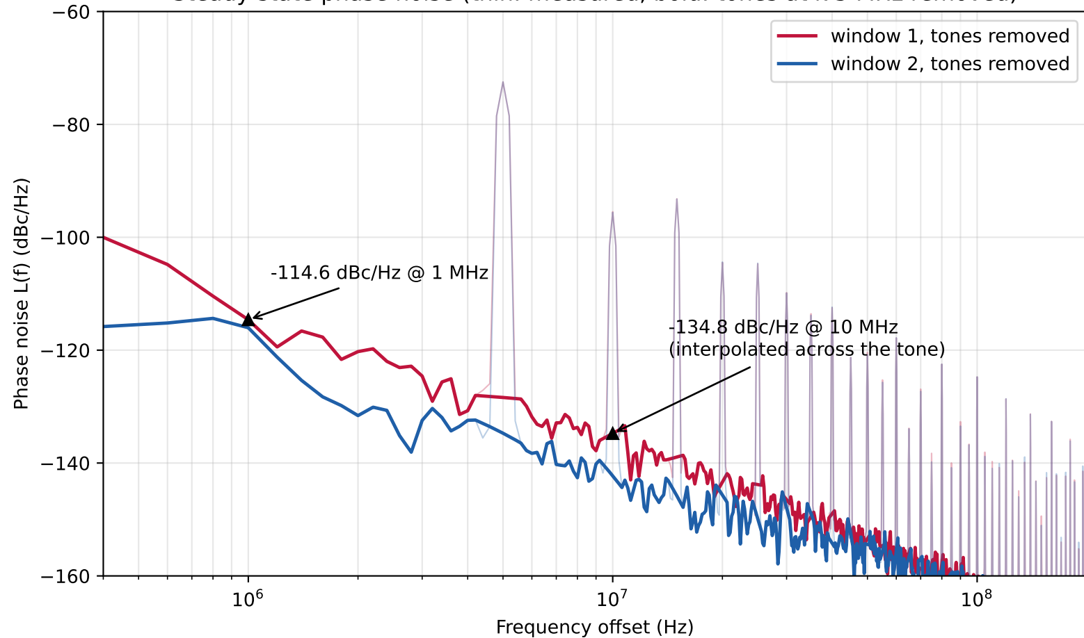
Steady-state phase noise (thin: measured, bold: tones at k \cdot 5 MHz removed)
