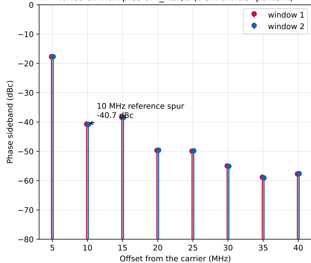
Tones at multiples of f_{\text{REF}}/2 (DSM divider pattern)
