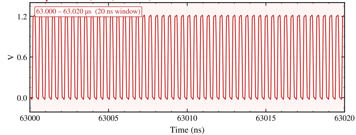
Output Clock (VCO, 2.4 GHz) — 20 ns zoom
