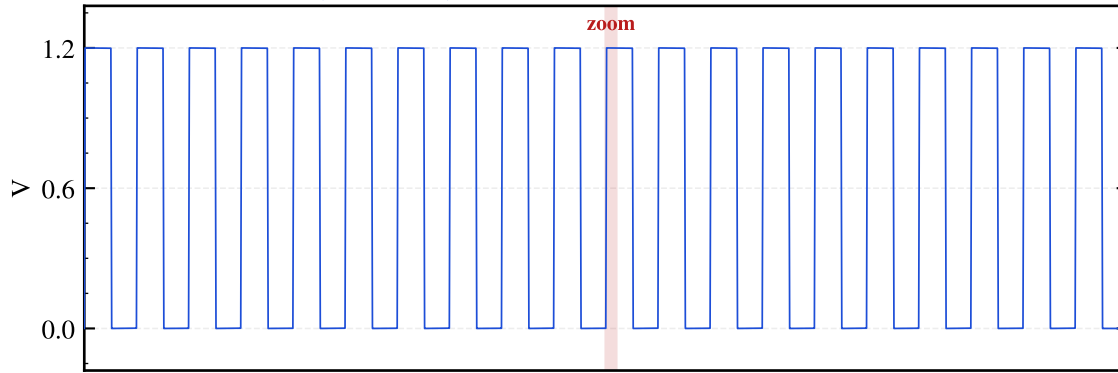
Feedback Clock (PFD in B)
